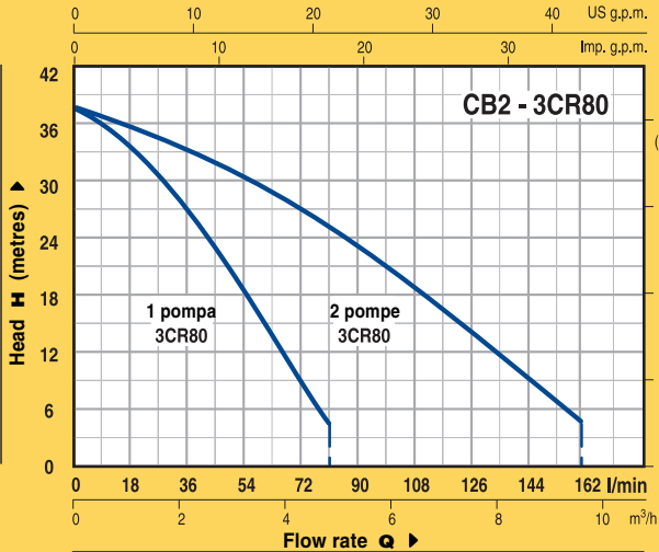
CURVES AND PERFORMANCE DATA AT n= 2900 1/min
