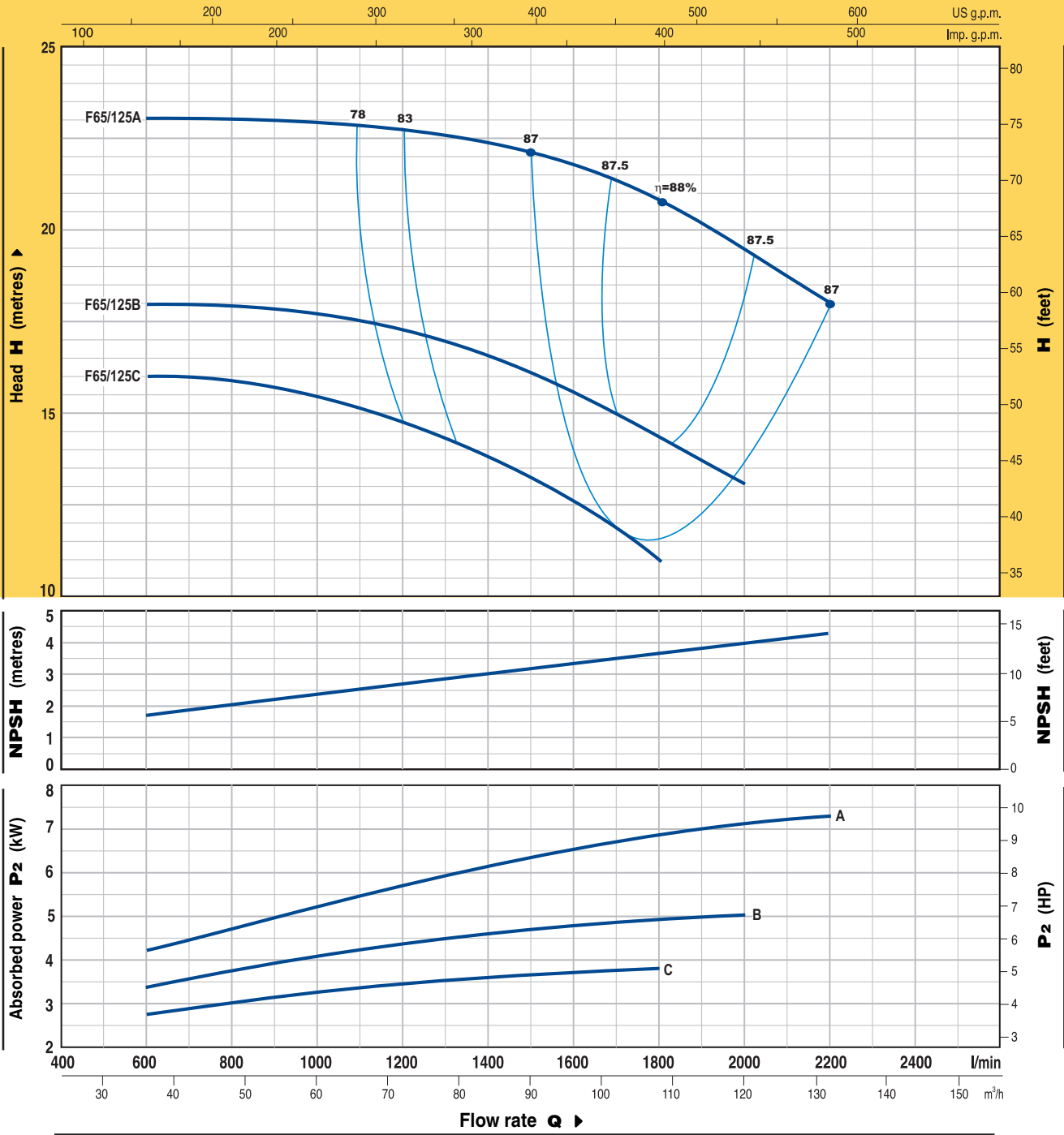
CURVES AND PERFORMANCE DATA AT n= 2900 1/min
