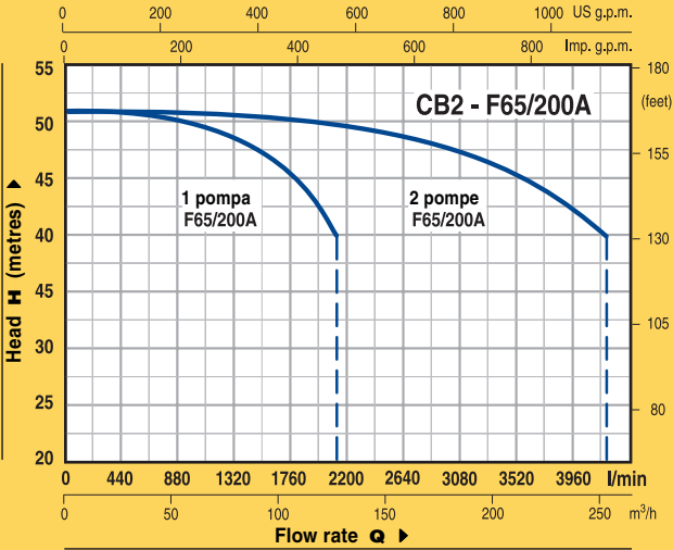
CURVES AND PERFORMANCE DATA AT n= 2900 1/min
